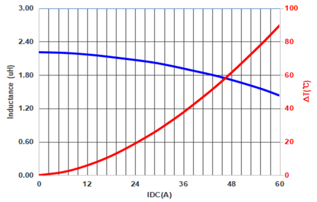
PIF1508A2R2MO
