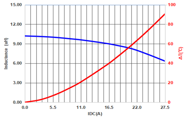
PIF1508A100MO
