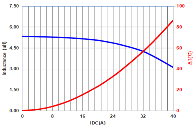
PIF1508A5R3MO
