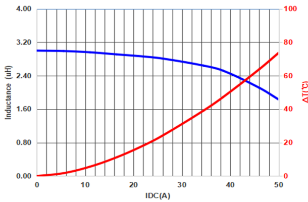
PIF1508A3R0MO
