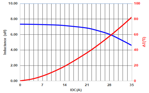
PIF1508A7R2MO
