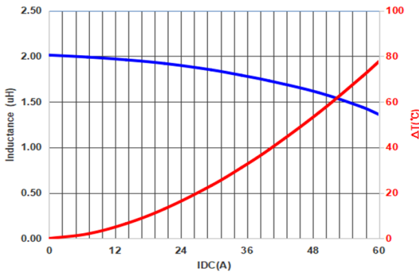
PIF1508A2R0MO
