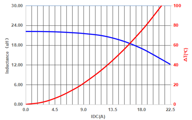
PIF1508A220MO
