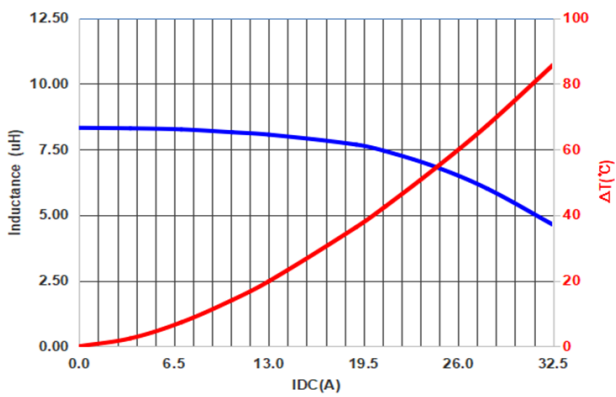
PIF1508A8R2MO
