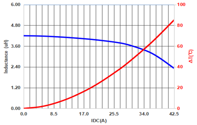
PIF1508A4R2MO
