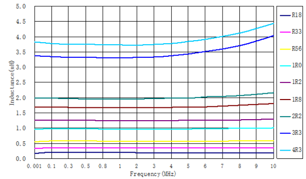
PIF0603A Series
