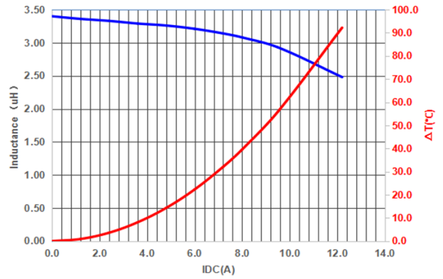
PIF0603A3R3MN
