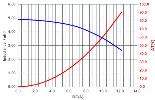
PIF0603A4R5MN
