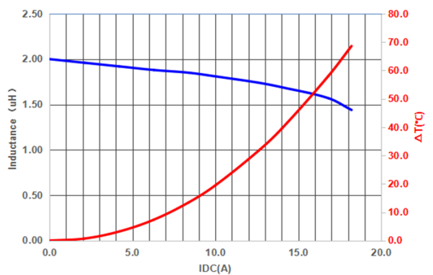
PIF0603A1R8MN
