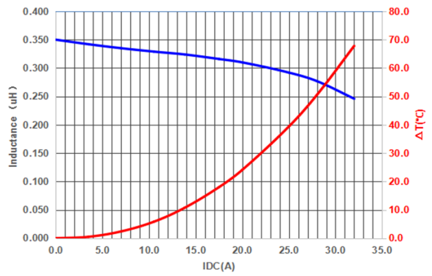
PIF0603AR33MN
