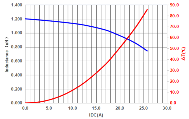
PIF0603A1R0MN
