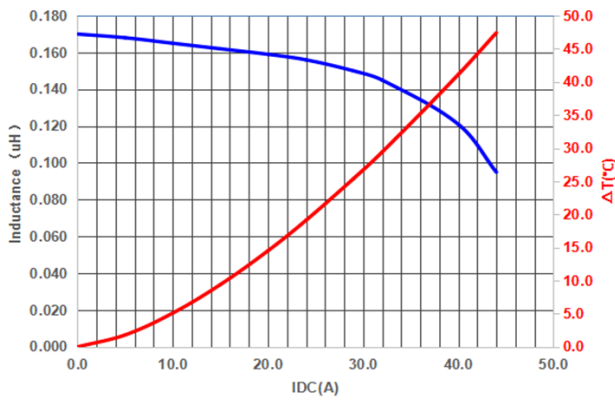
PIF0603AR18MN
