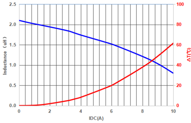
PIF0402LR2R0MN
