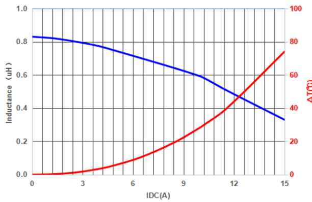
PIF0402LRR82MN
