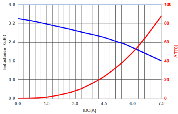
PIF0402LR3R3MN
