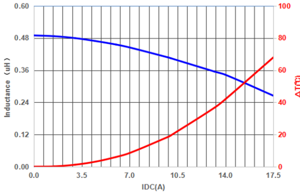
PIF0402LRR47MN
