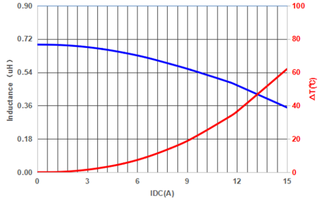
PIF0402LRR68MN
